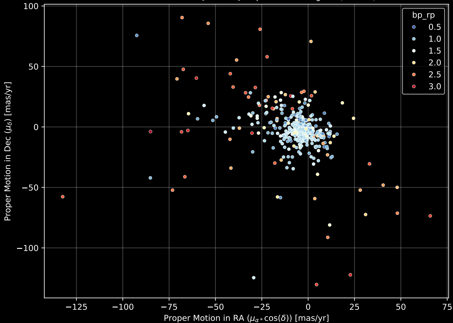
APOGEE DR17 Field: [040+45] Proper Motion Diagram (n= 433)
