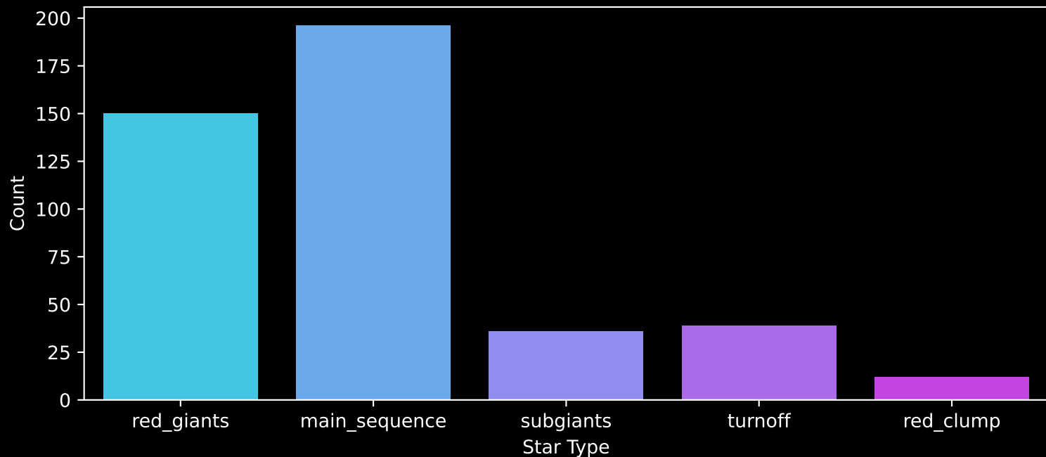
APOGEE DR17 Field: [040+45] Count plot of Star Type
