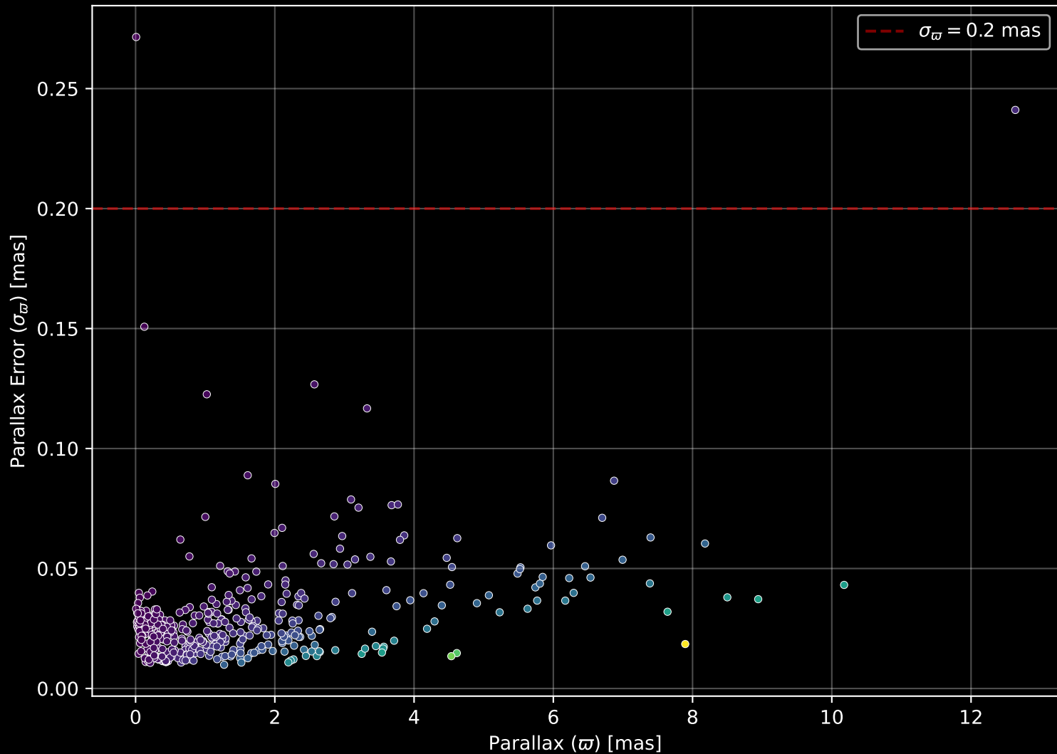
APOGEE DR17 Field: [040+45] Parallax Quality (n= 433)
