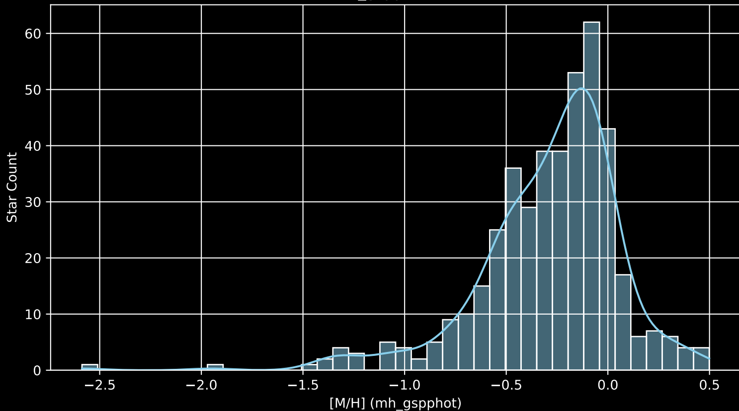
APOGEE DR17 Field: [040+45 [M/H] (mh_gspphot) (n= 432)
