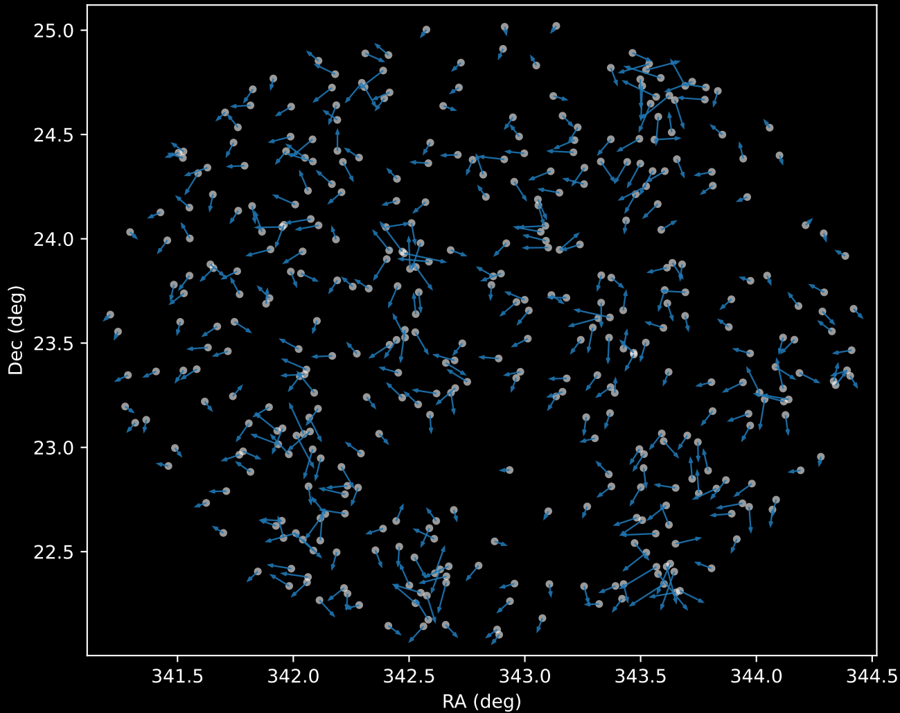
APOGEE DR17 Cluster 0 Proper Motion Vectors (n=405)
