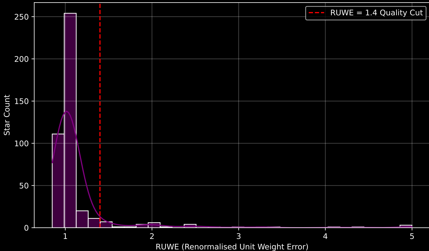
GAPOGEE DR17 Field [040+45] RUWE Distribution (n= 429)
