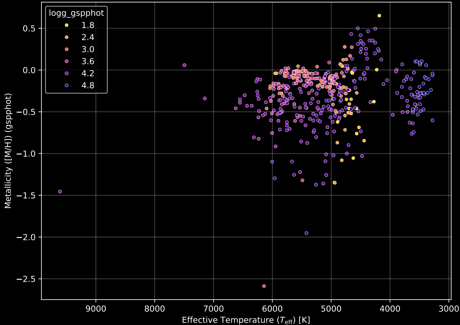
APOGEE DR17 Field: [040+45] Stellar Population Parameters (n= 433)
